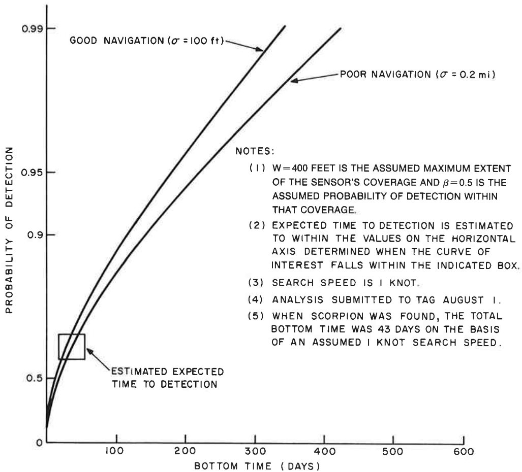
FIGURE 3. Probability of detection for one ship using magnetometer and sonar ( W=400 ft and \beta=0.5 )
