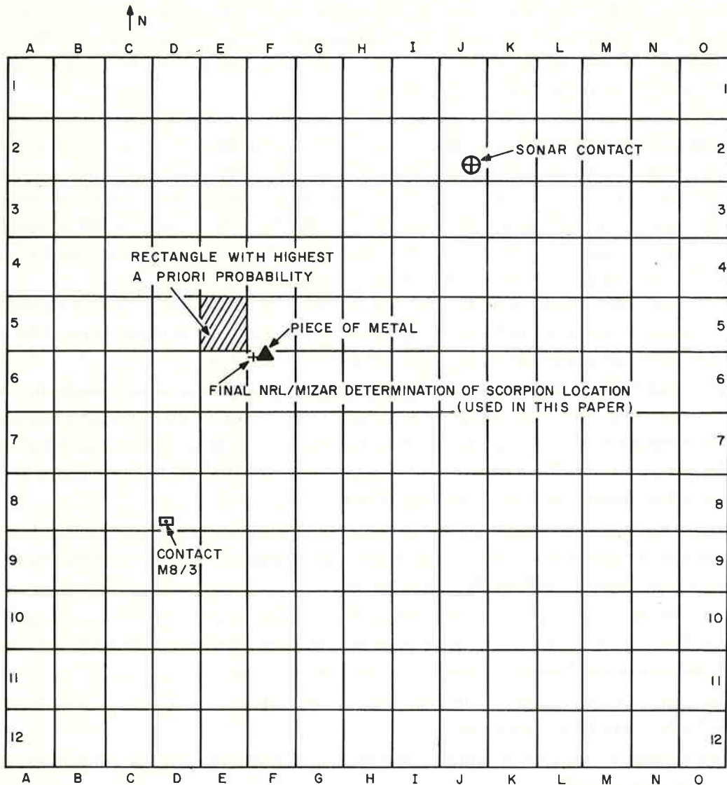
FIGURE 1. Scorpion search grid
