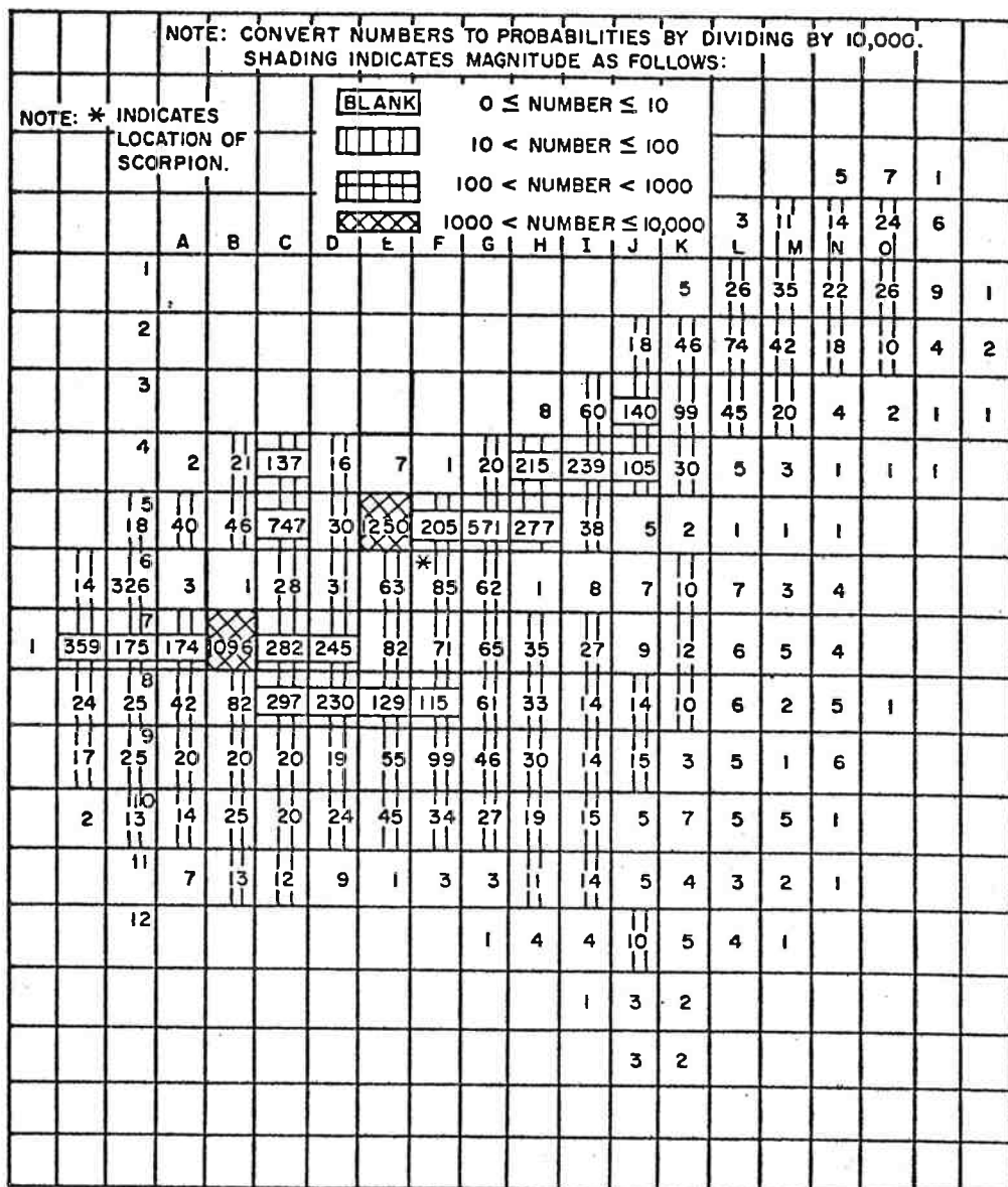
FIGURE 2. Overall A Priori distribution for Scorpion search
